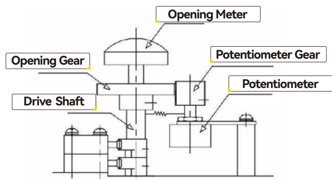
(Drawing 5)
